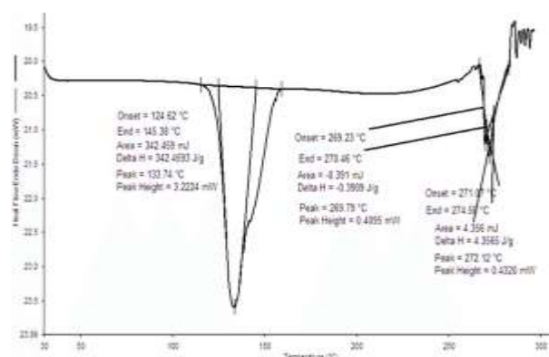
Figure 3: DSC Study of Oxiconazole with HPMC
