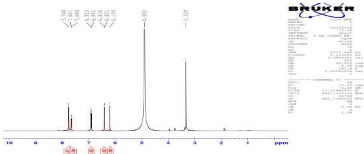
Figure 7: 1H NMR data of luteolin
