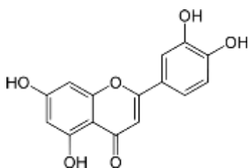
Luteolin
