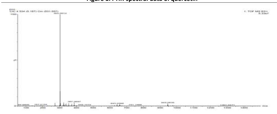
Figure 2: LC-Q-TOF data of quercetin
