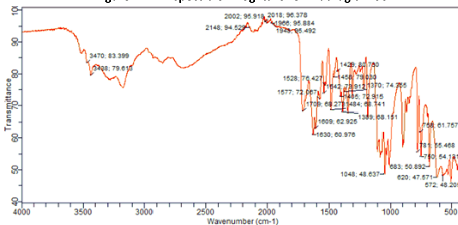
Figure 3: FTIR spectra of Pioglitazone + Ethyl cellulose
