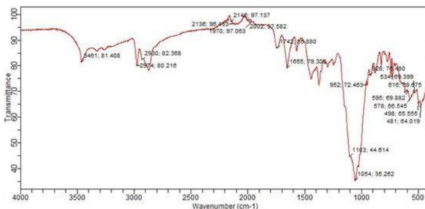
Figure 1: FTIR spectra of Pioglitazone hydrochloride
