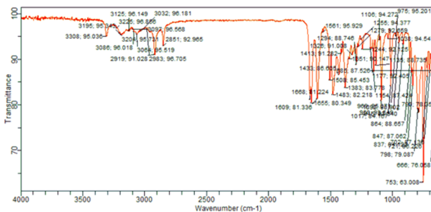
Figure 2: FTIR spectra of Pioglitazone + Eudragit L100
