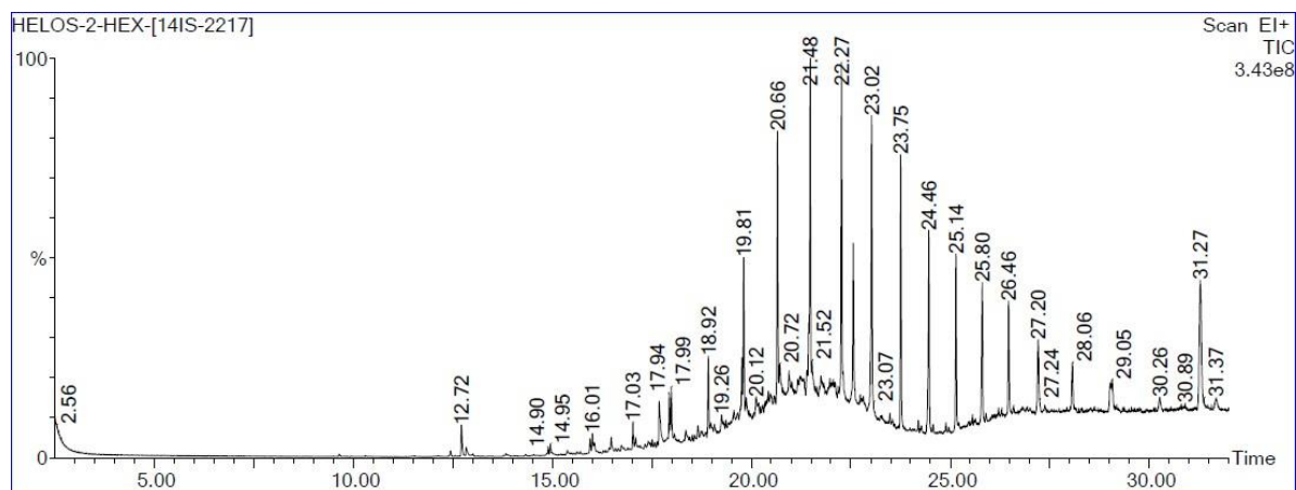
Figure 2: GC-MS of the dry leaves
