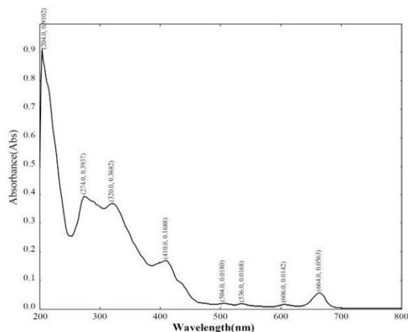
Figure 4: Shows UV Analysis of Ormocarpum sennoides DC
