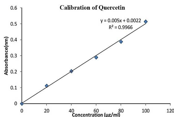
Figure 1: Shows total flavonoid content (Quercetin standard) of Ormocarpum senoides DC
