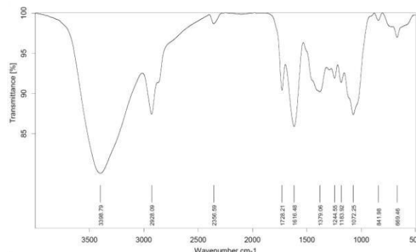
Figure 5: Shows IR Analysis of Ormocarpum sennoides DC
