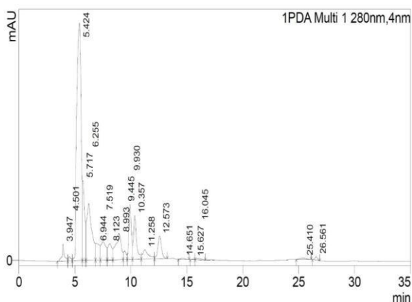
Figure 3: HPLC analysis of Ormocarpum sennoides DC
