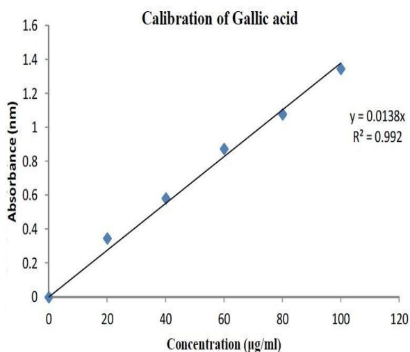
Figure 2: Shows total phenolic content (Gallic acid standard) of Ormocarpum sennoides DC
