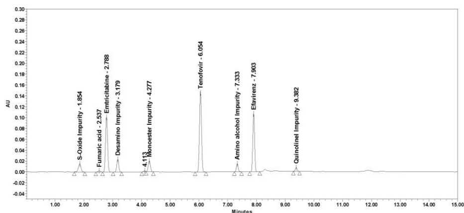
Figure 4: Typical Chromatogram of Standard solution Spiked with Known Degradent impurities
