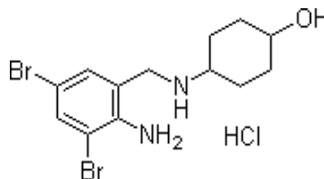
Figure 2: Structure of ambroxol hydrochloride
