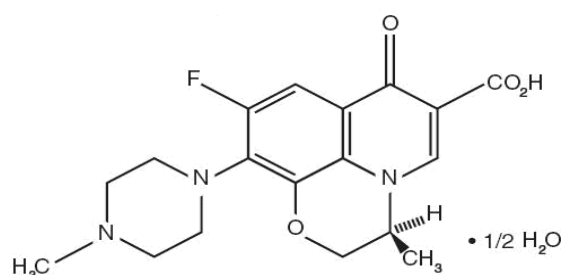
Figure 1: Structure of levofloxacin
