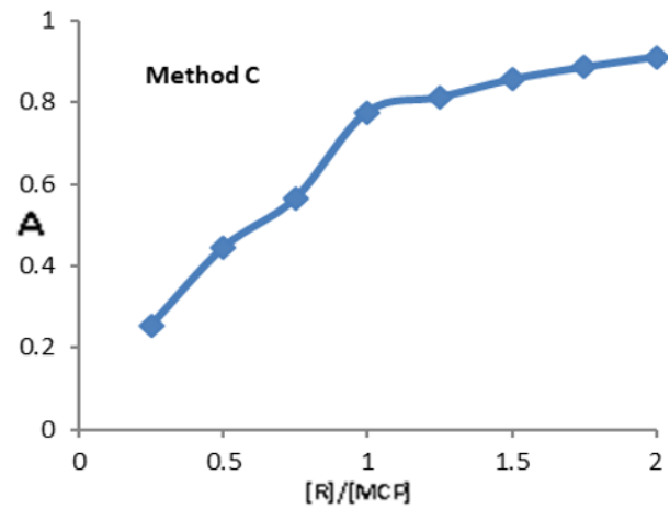
Figure 21: Mole ratio method for method C
