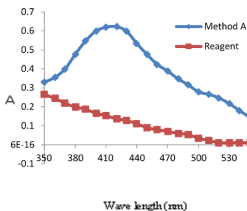
Figure 2: Absorption spectra of metoclopramide hydrochloride azo dye with the resorcinol reagent (5.0 \mu\text{g}/\text{mL} )
